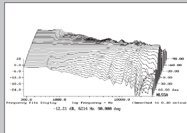
Fig.4 GoldenEar Triton Two, lateral response family at 50", normalized to response on tweeter axis, from back to front: differences in response 90-5° off axis, reference response, differences in response 5-90° off axis.
