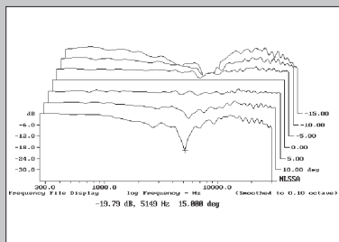
Fig.5 GoldenEar Triton Two, vertical response family at 50", normalized to response on tweeter axis, from back to front: differences in response 15-5° above axis, reference response, differences in response 5-15° below axis.
